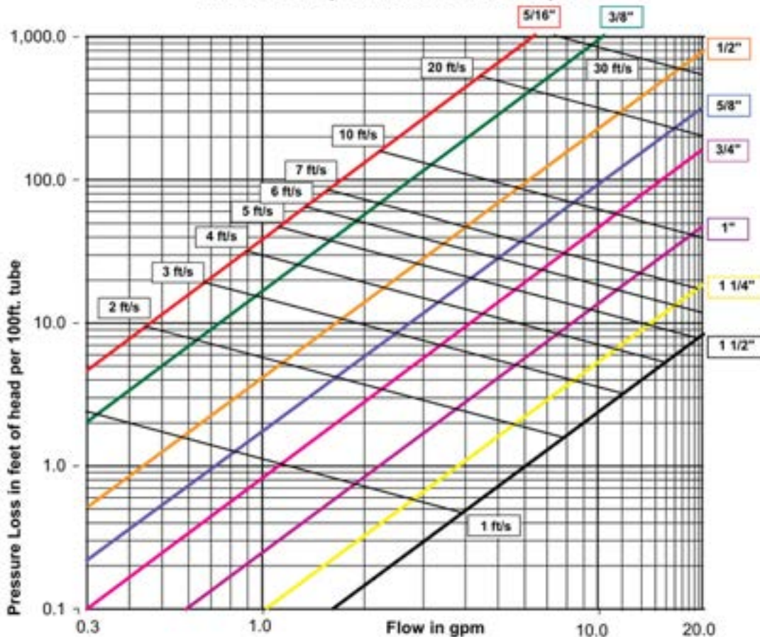
Pressure Drop Chart PEOC-PLUS Pipes
