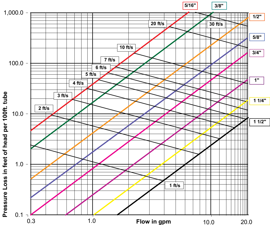
Pressure Drop Chart PEOC-PLUS Pipes
